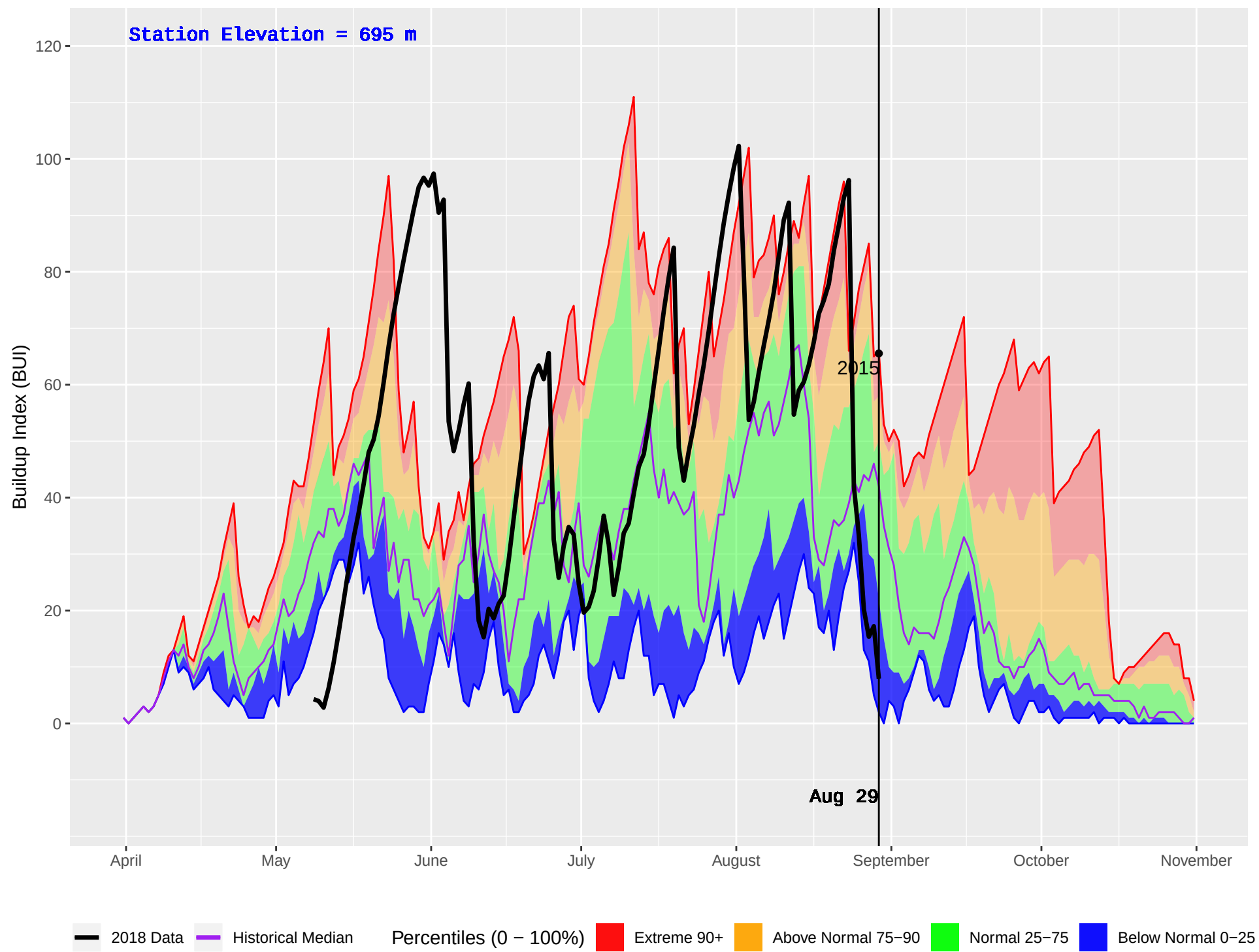
BLUE RIVER 2 (1108) : Historical (2011–2016) and Current (2018) Daily Buildup Index (BUI)
