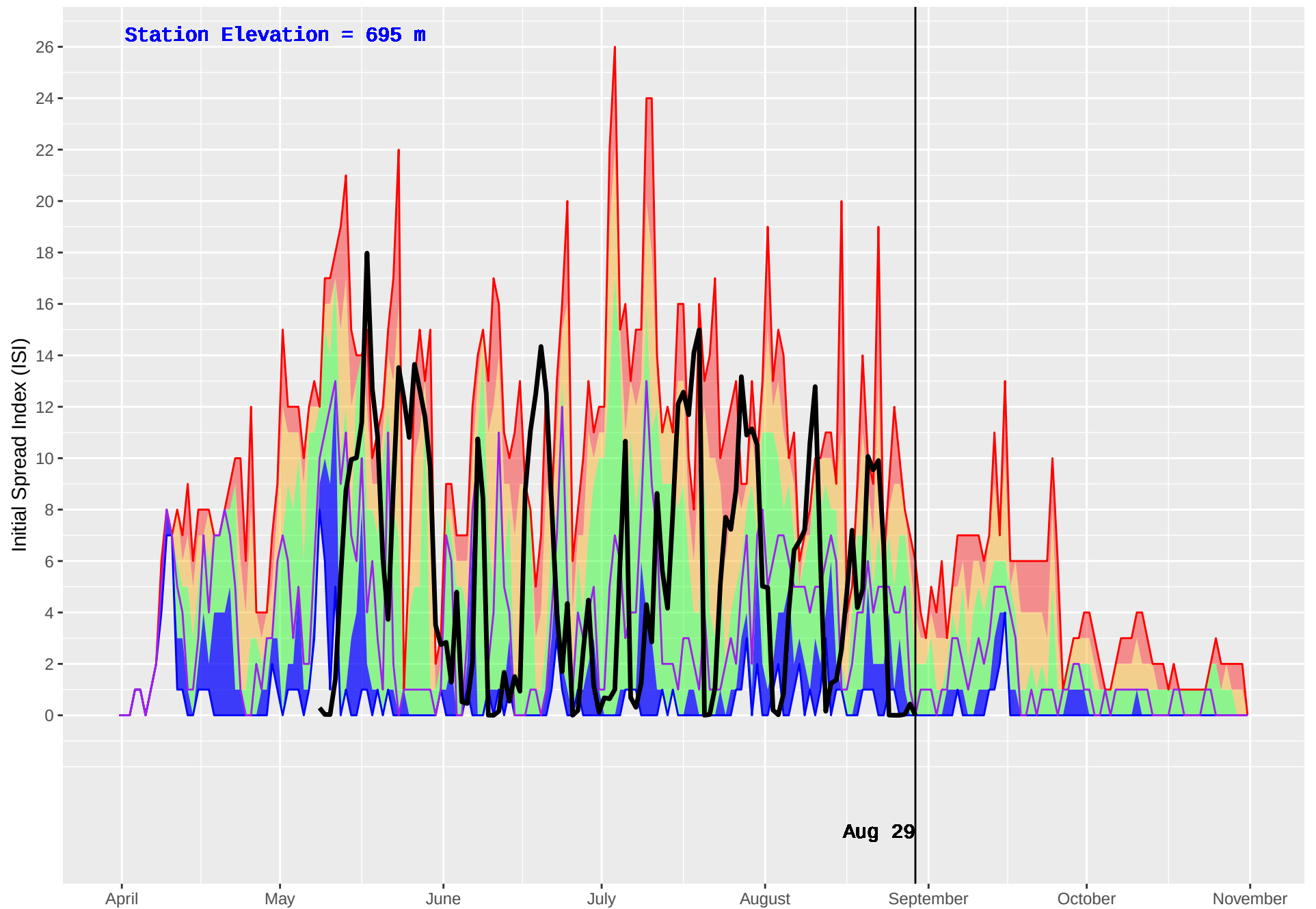
BLUE RIVER 2 (1108) : Historical (2011–2016) and Current (2018) Daily Initial Spread Index (ISI)
