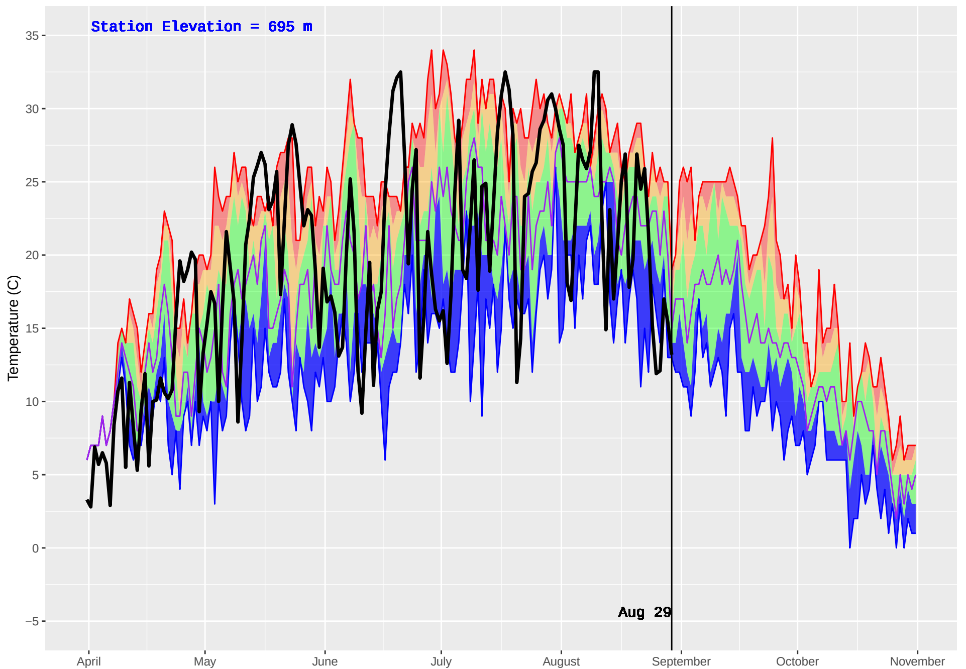
BLUE RIVER 2 (1108) : Historical (2011–2016) and Current (2018) Daily Temperature
