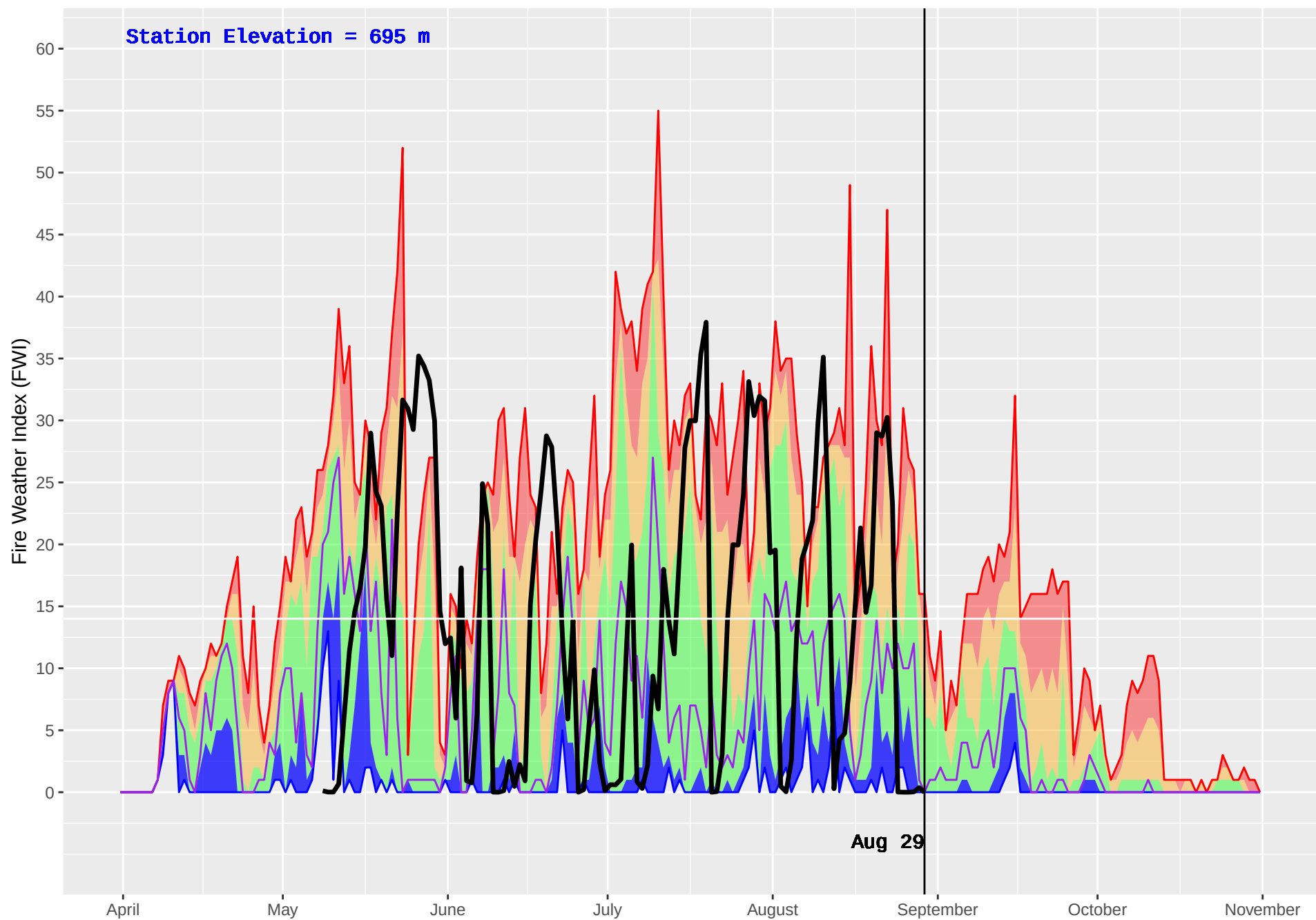
BLUE RIVER 2 (1108) : Historical (2011–2016) and Current (2018) Daily Fire Weather Index (FWI)
