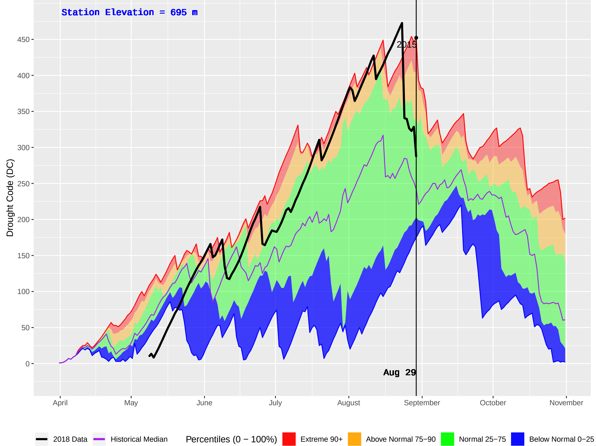
BLUE RIVER 2 (1108) : Historical (2011–2016) and Current (2018) Daily Drought Code (DC)
