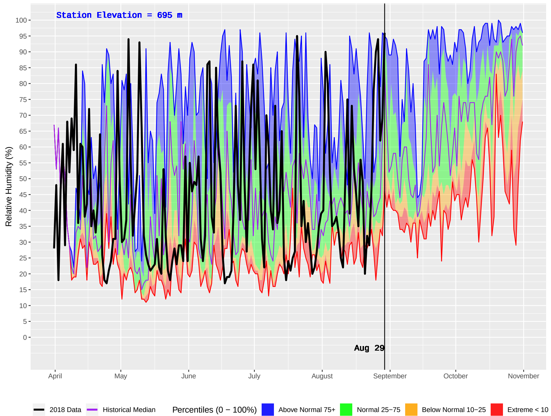
BLUE RIVER 2 (1108) : Historical (2011–2016) and Current (2018) Daily Relative Humidity
