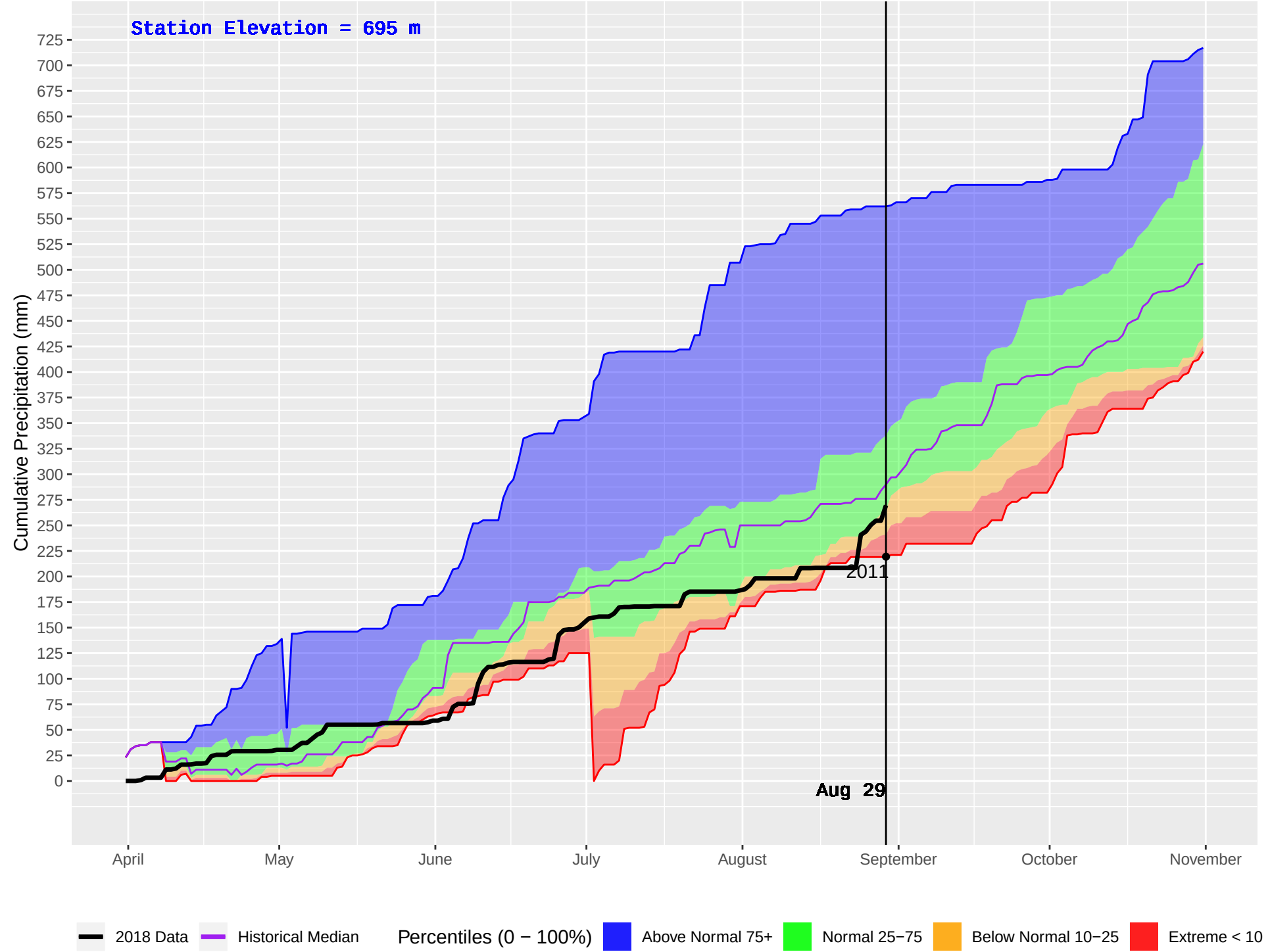
BLUE RIVER 2 (1108) : Historical (2011–2016) and Current (2018) Daily Cumulative Precipitation
