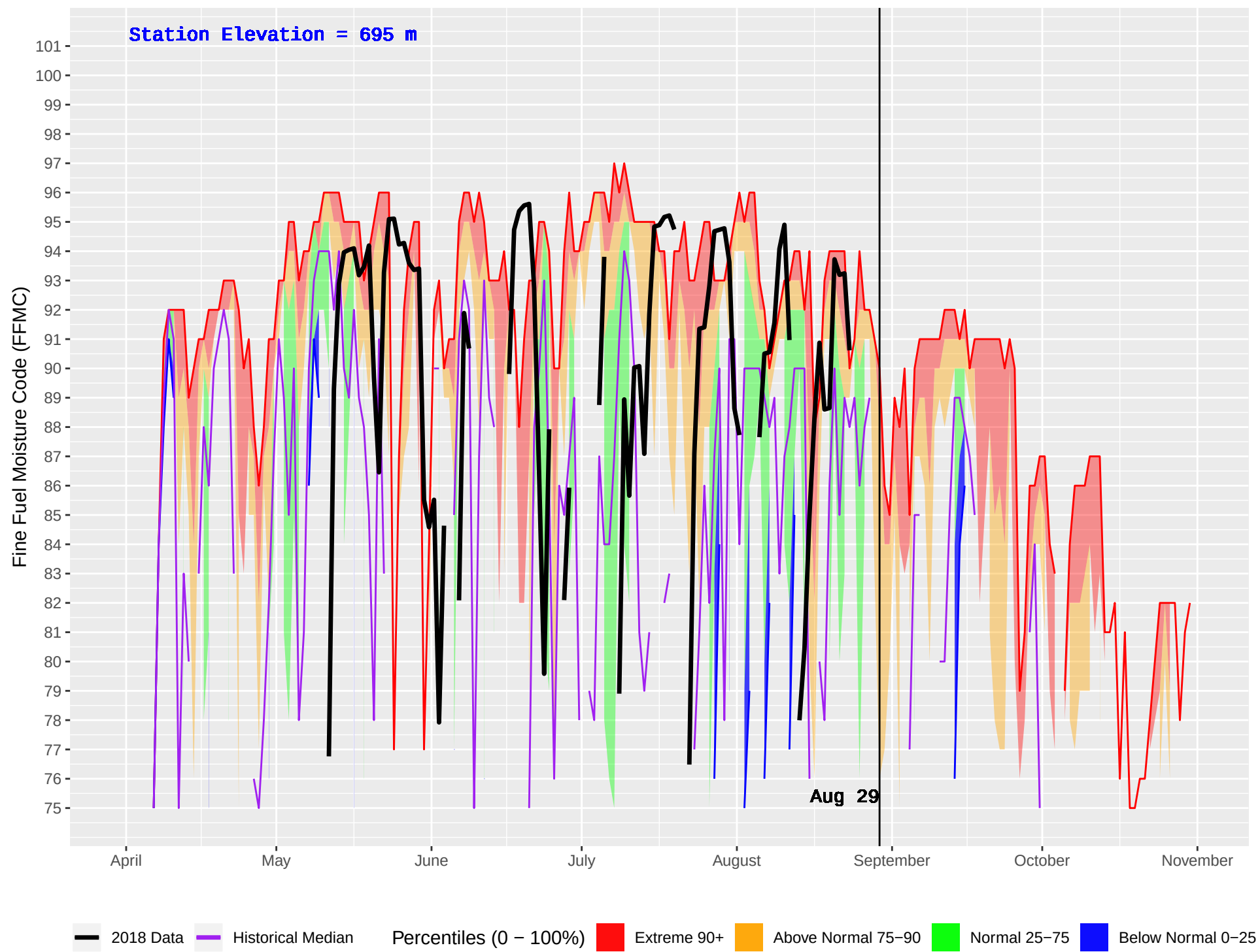
BLUE RIVER 2 (1108) : Historical (2011–2016) and Current (2018) Daily Fine Fuel Moisture Code (FFMC)
