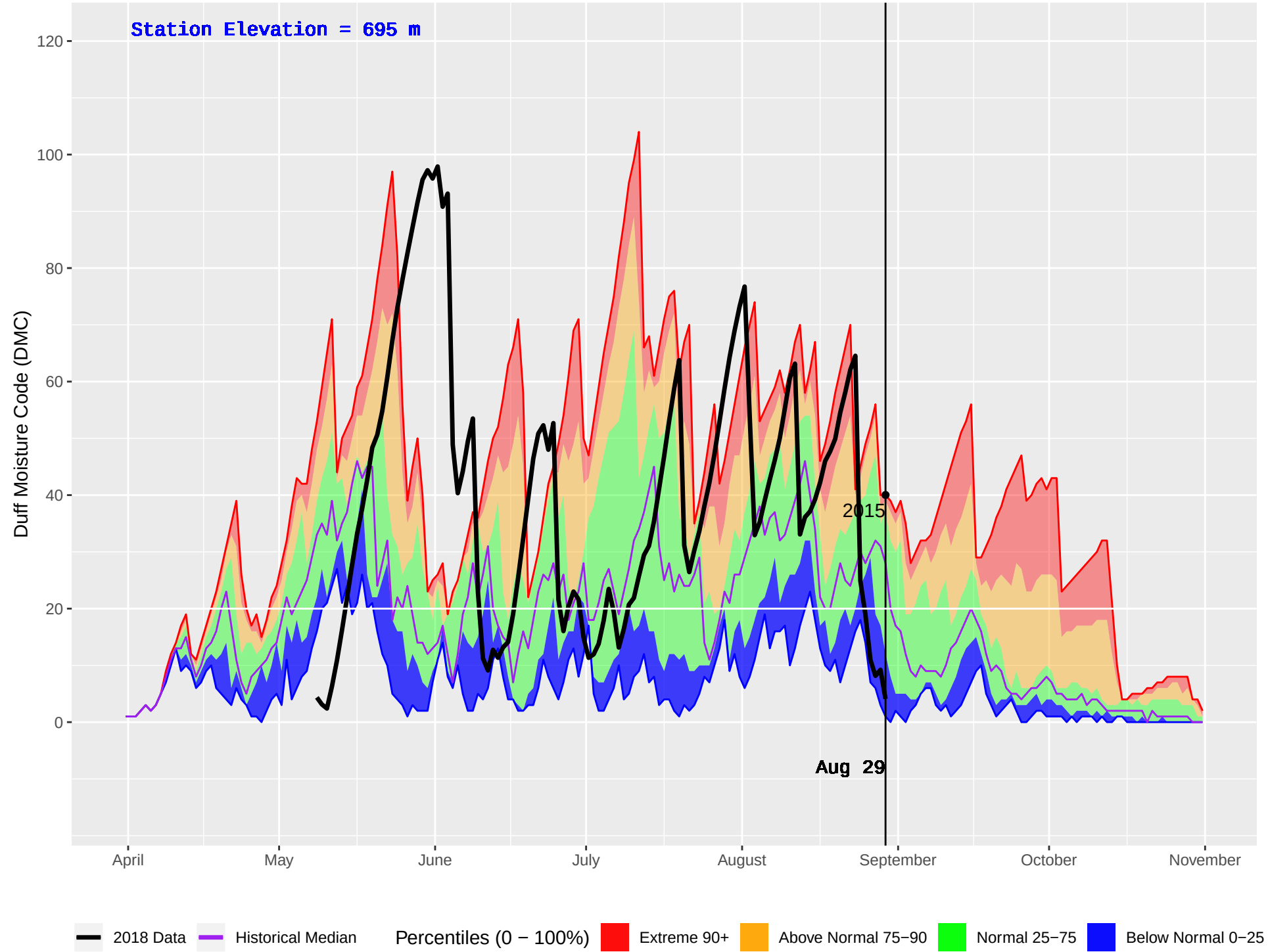
BLUE RIVER 2 (1108) : Historical (2011–2016) and Current (2018) Daily Duff Moisture Code (DMC)
